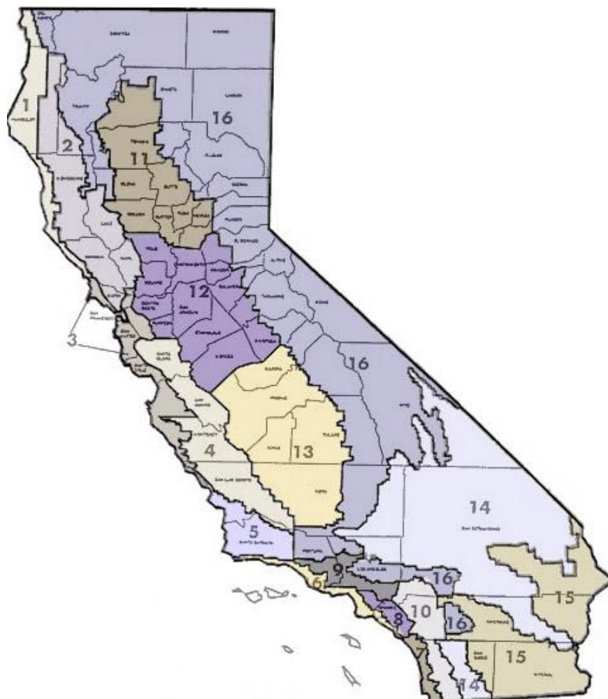
Figure 2-3: California Building Climate Zones
